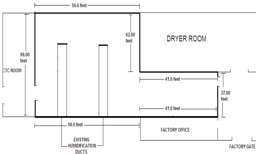
Fig: Diagram of Fermenting Room with necessary specifications.
